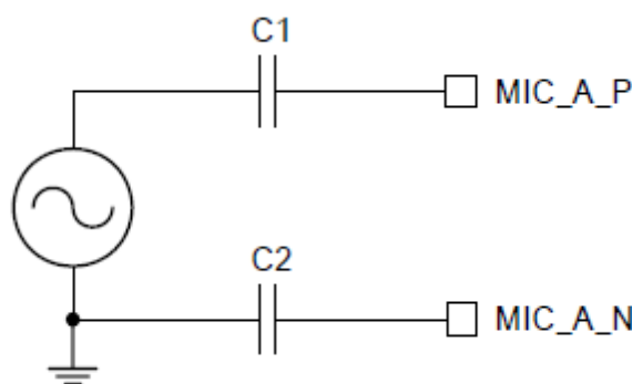
Single-Ended Input (Single Channel Shown)
