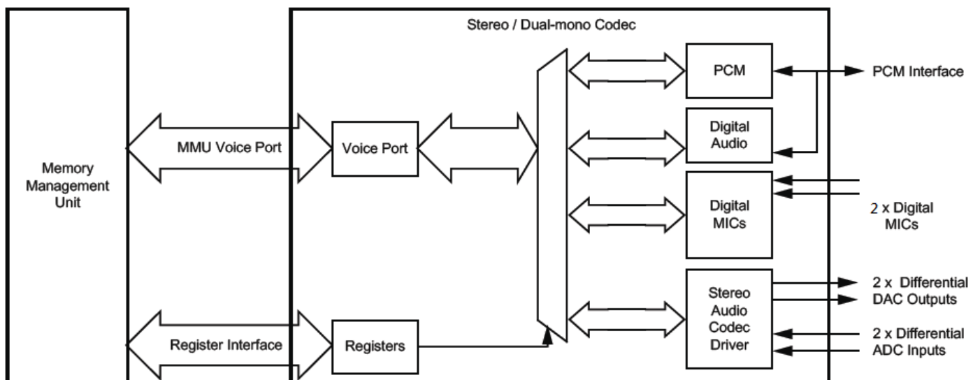
Audio Interface
