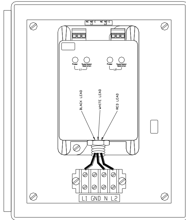
ENCLOSURE SHOWN WITH DOOR REMOVED
